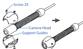
Figure 9. Install 46 Support Guides
