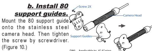
Figure 10. Install 80 Support Guides
