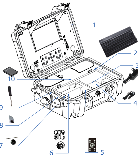
Figure 5. Package Contents
